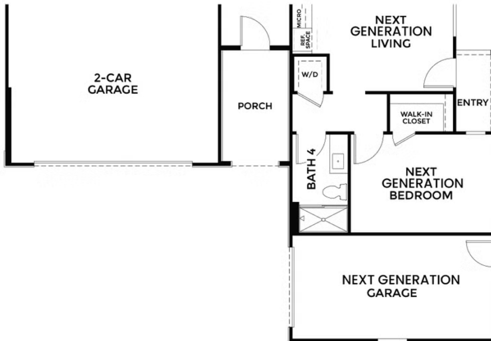
ELEVATION TRADITIONAL FIRST FLOOR
