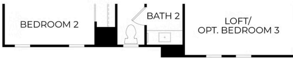
ELEVATION C SECOND FLOOR (SAME AS ELEVATION A)
