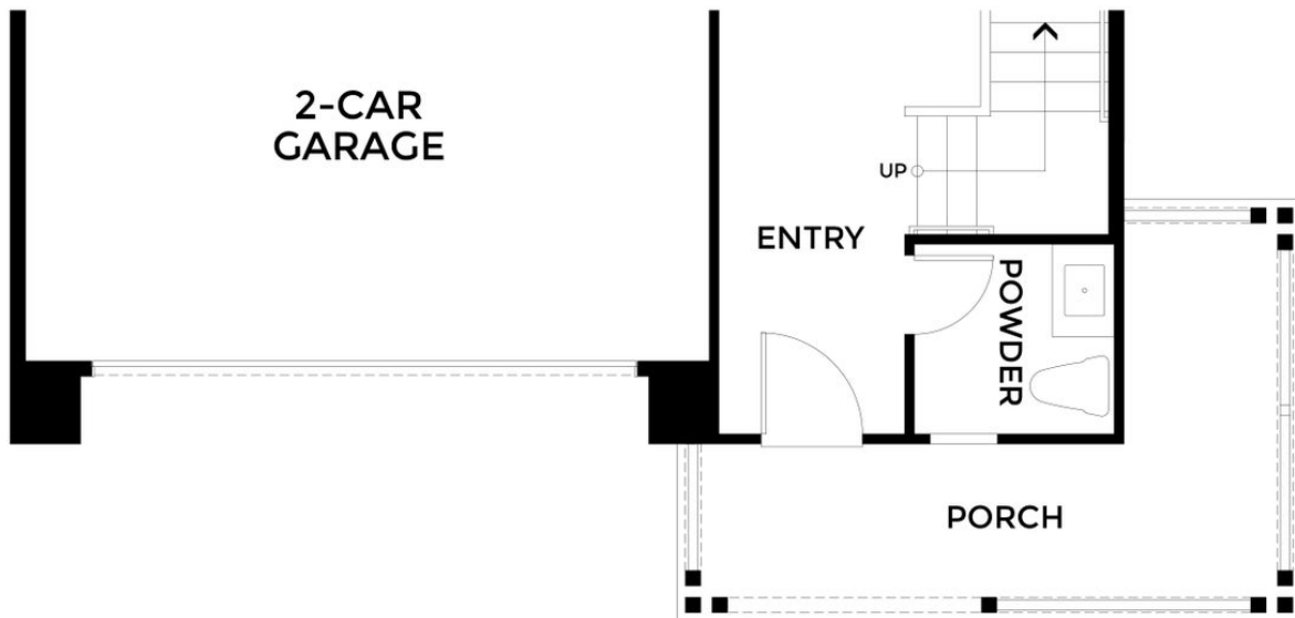
ELEVATION A FIRST FLOOR WRAP PORCH
